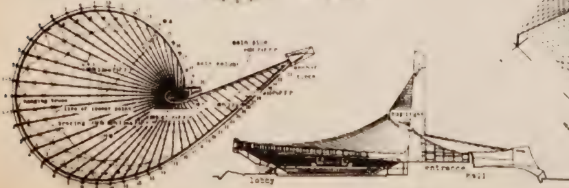
Figure 1. Roof plan and section.
